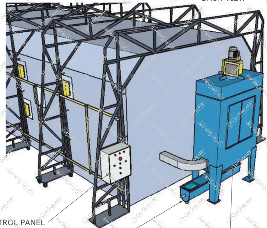
BACK VIEW
