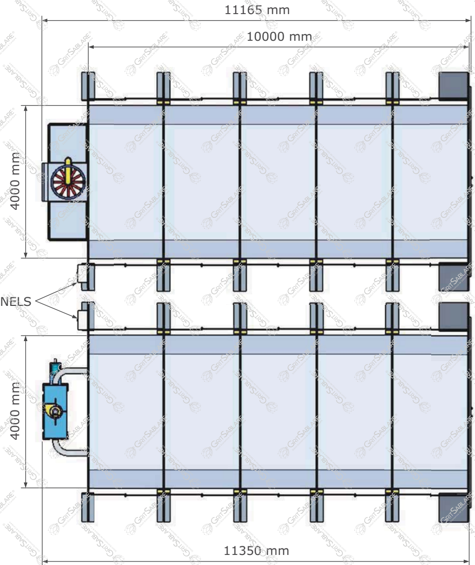
PLAN VIEW
